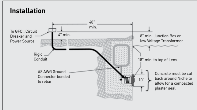
Installation requires meeting electrical requirements and standard local codes.
