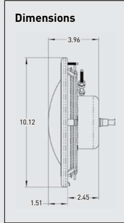
Drawing shows innovative lens and reflector designs which combine to provide superior light beam distribution.
