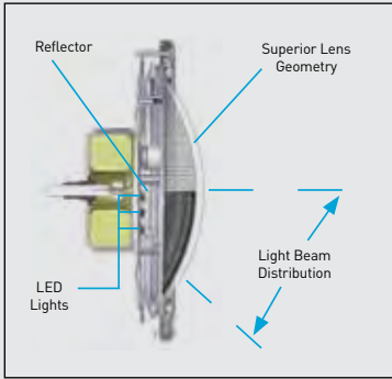
Drawing shows innovative lens and reflector designs which combine to provide superior light beam distribution.
